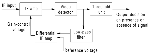
Figure D7 Simplified adaptive detection.
