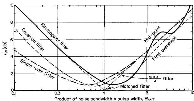
Figure L25 Filter matching loss vs. filter noise bandwidth B_{nh} for rectangular pulse of with \tau with different filters (from Barton, 1969, Fig. 3.17, p. 84).
