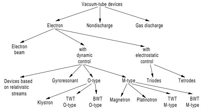
Figure D36 Classification of vacuum-tube devices.
