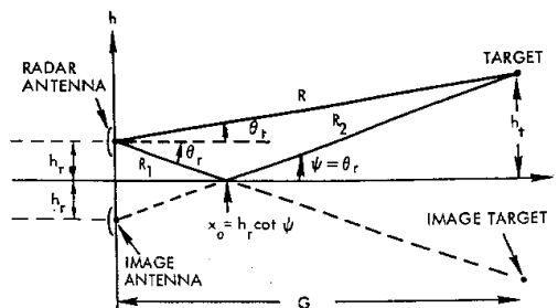
Figure P18 Multipath geometry over flat Earth.
