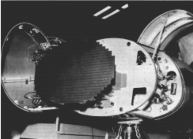
Figure R5 AN/APG-66 AI radar mounted in nose of F-16 fighter.
