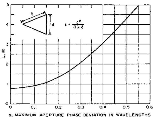
Figure A61 Loss correction for phase error in conical horns (from Johnson, 1993, Fig. 15.11, p. 15.17, reprinted by permission of McGraw-Hill).
