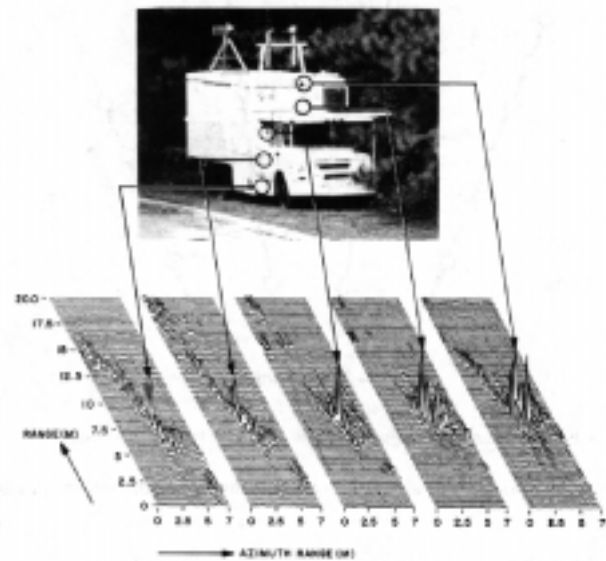
Figure I1 Image created using focused beam antenna (from Currie, 1989, Fig. 10.16, p. 398).
