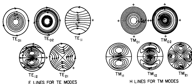
Figure W18 Field configurations for circular waveguide (from Johnson, 1984, Fig. 42-14, p. 42-33, reprinted by permission of McGraw-Hill).
