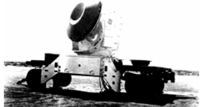
Figure R22 Nike Hercules monopulse fire control radar.
