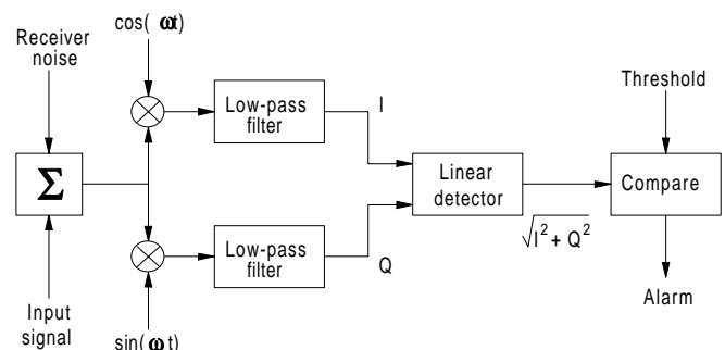
Figure D21 I/Q detection (after Blake, 1980,
