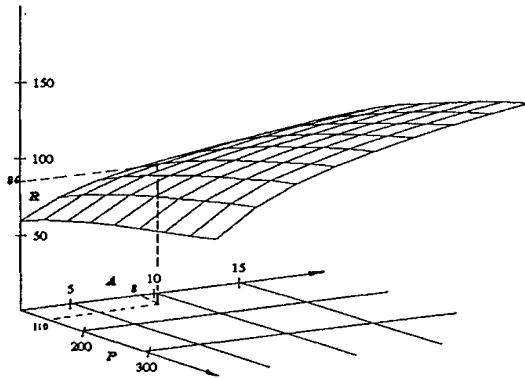
Figure T17 Average power vs. antenna aperture, S-band search radar (from Barton, 1991, Fig. K.1, p. K-6).
