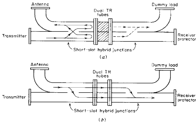
Figure D57 Balanced duplexer using dual TR tubes and two short-slot hybrid junctions: (a) transmit condition (b) receive condition (from Skolnik, 1980, Fig. 9.6, p. 361, reprinted by permission of McGraw-Hill).
