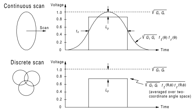
Figure L19 Definition of beamshape loss for one-coordinate continuous scan and discrete-position raster scan.
