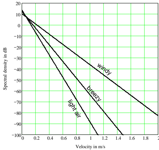
Figure C27 Spectra of windblown tree clutter.
