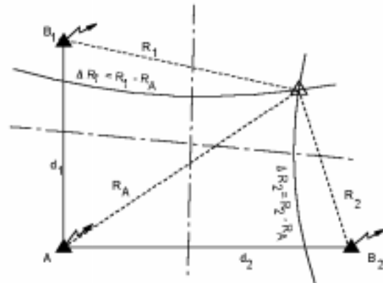
Figure N3 Range-difference navigation method.
