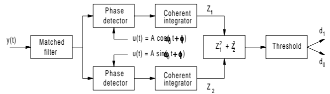
Figure D10 Filter detector.
