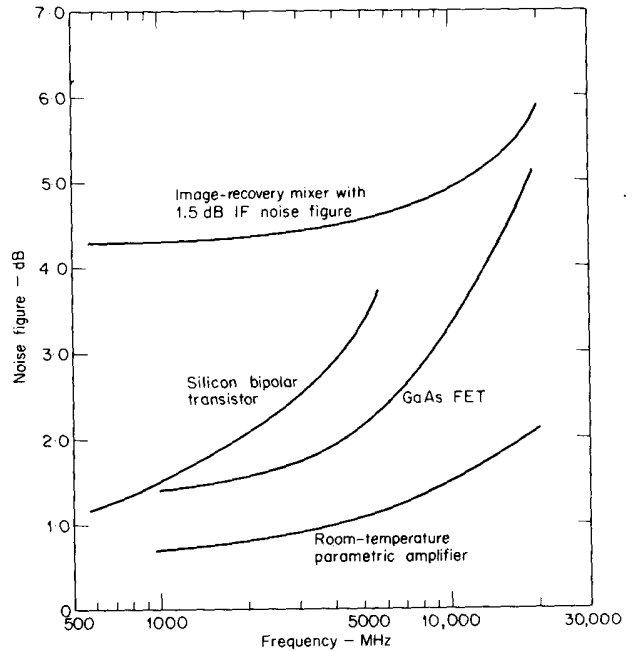
Figure R98 Noise figures for typical receiver front ends (from Skolnik, 1980, Fig. 9.4, p. 351, reprinted by permission of McGraw-Hill).
