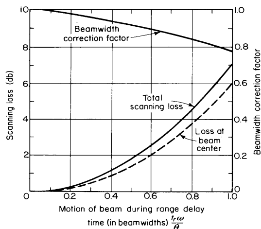
Figure L30 Scanning loss vs. scan speed (from Barton, 1964, Fig. 5.6, p. 150).
